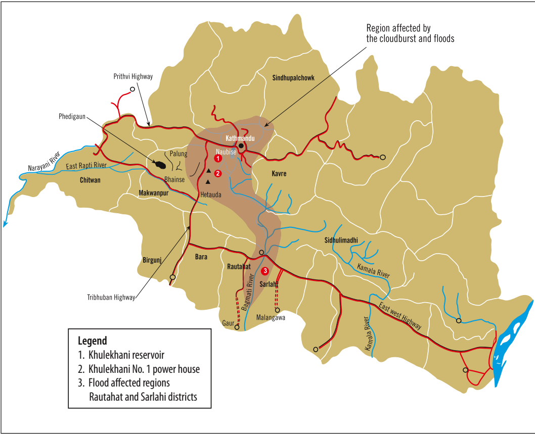
FIGURE 7.2 Koshi embankment
